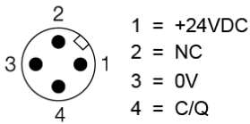
IO-Link M12 interface 4-pin male
