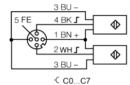
Digital input M12 interface
