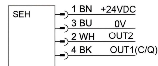
Wiring diagram
