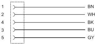
M12 Circuit Diagram
