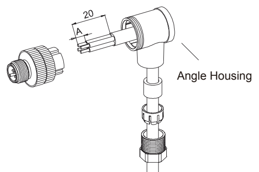
Connection mode 4/5-pin, Screw/clamp connection
